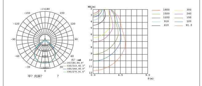
Light Distribution Curve
